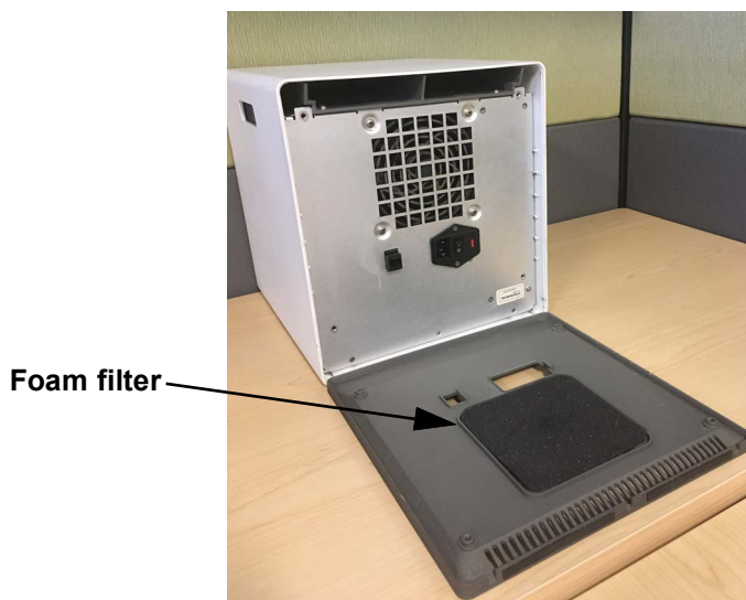
Figure 9-15. Foam Filter in Older GX-IV
